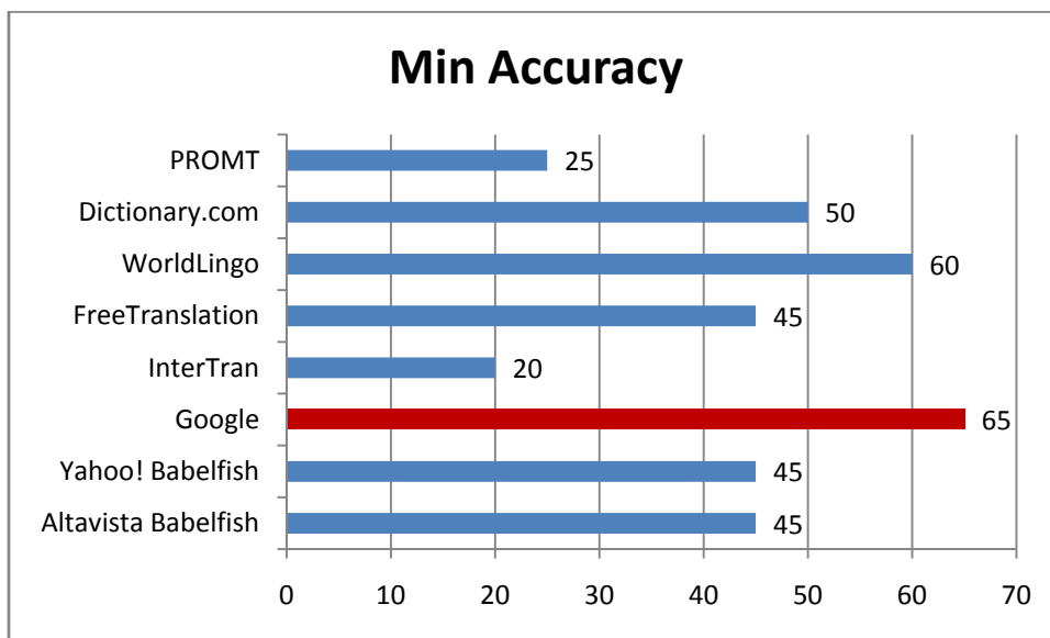
Figure 3-3. Minimum accuracy graph in Spanish-English Benchmark.
