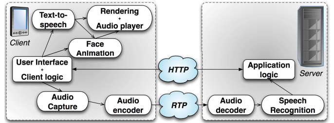
Figure 3: Client-server configuration that uses the server for application-logic processing and for speech recognition. Results of the recognition process are directly provided to the application-logic module. The client side is used for text-to-speech processing, face animation and their synchronization. This architecture is supported by our framework.
