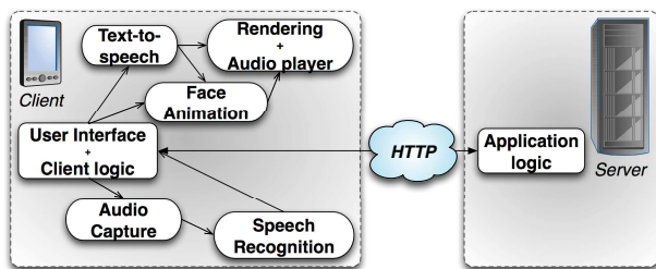
Figure 4: Client-server configuration that uses the server side for application-logic processing only. Our framework supports this type of configuration. It is suitable only for mobile devices with great computational power. Also this configuration is convenient in situations where only low bandwidth is available.
