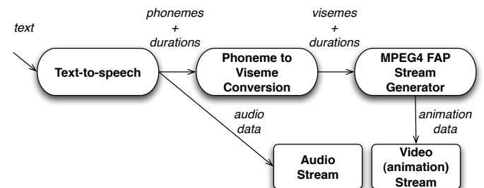
Figure 7: Process for generating face animation based on phonemes durations.
