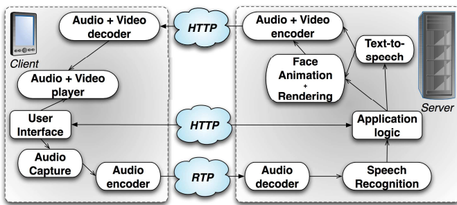
Figure 2: Video-streaming architecture is convenient for less powerful mobile phones with fast Internet connection, because it delegates most of the application work to a remote server. It can be easily implemented as platform-independent. We did not include such architecture in our framework, because it is energetically inefficient.
