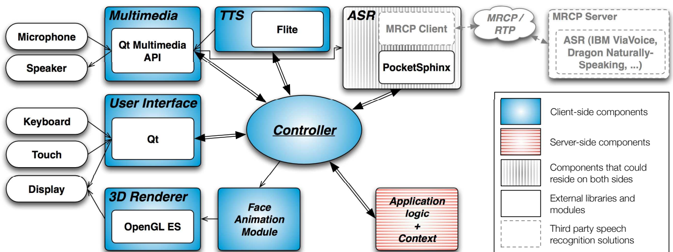
Figure 8: Framework architecture
