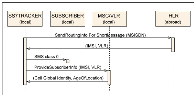
Figure 2: Messageflow for obtaining location of an inroamer
